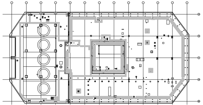
ROOF PLAN—WEST TOWER SCALE: 1/8" = 1'-0"
