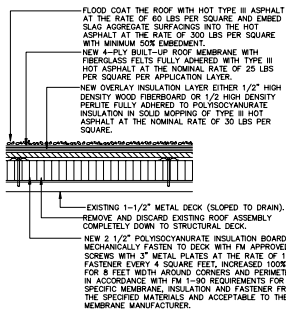
A TYPICAL ROOF ASSEMBLY "A" (AREAS A, B, & C) SCALE: NTS
