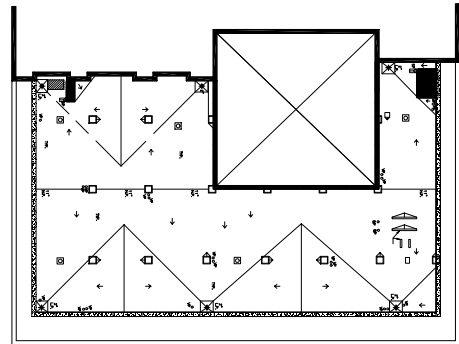
1 PARTIAL ROOF PLAN - ROOF AREA 6B SCALE: 1/8"=1'-0" SIXTH FLOOR SOUTH
