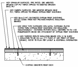
A1 ROOF ASSEMBLY #1 SCALE 1/8 FILE #8087-A1
