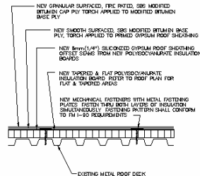
A2 ROOF ASSEMBLY #2 SCALE 1/8 FILE #8087-A2
