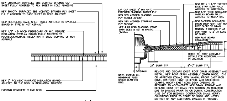
B TYPICAL ROOF ASSEMBLY 'B' NOT TO SCALE
